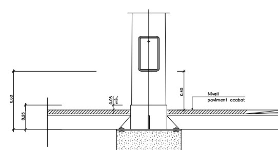
Columna i plaques base
