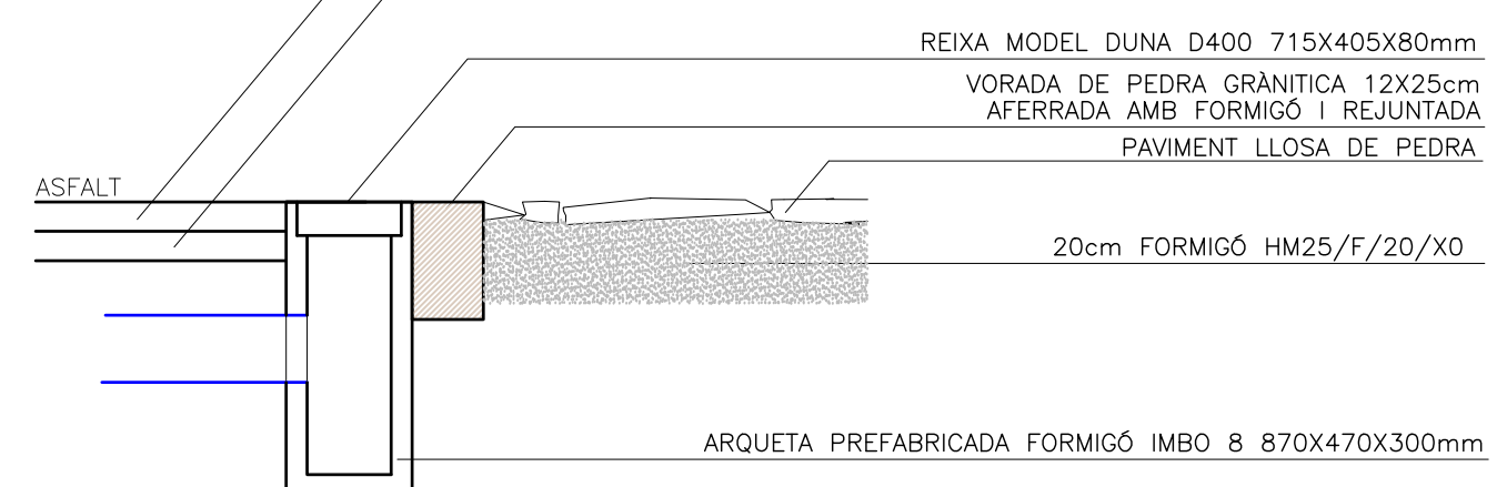
DETALL EMBORNAL E 1:20
