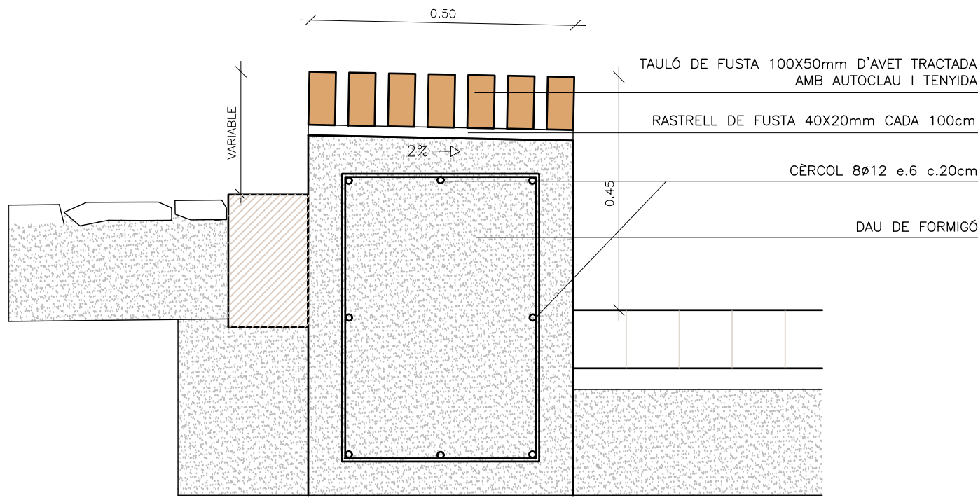
DETALL BANC E:1/10
